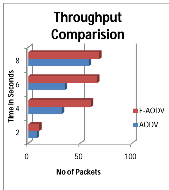
Fig 4: Throughput
